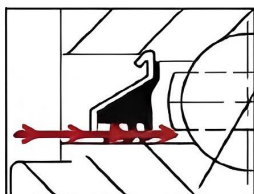
Bearing with 3 Lips
