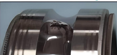
effect on raceway
