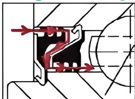
Bearing with 6 Lips
